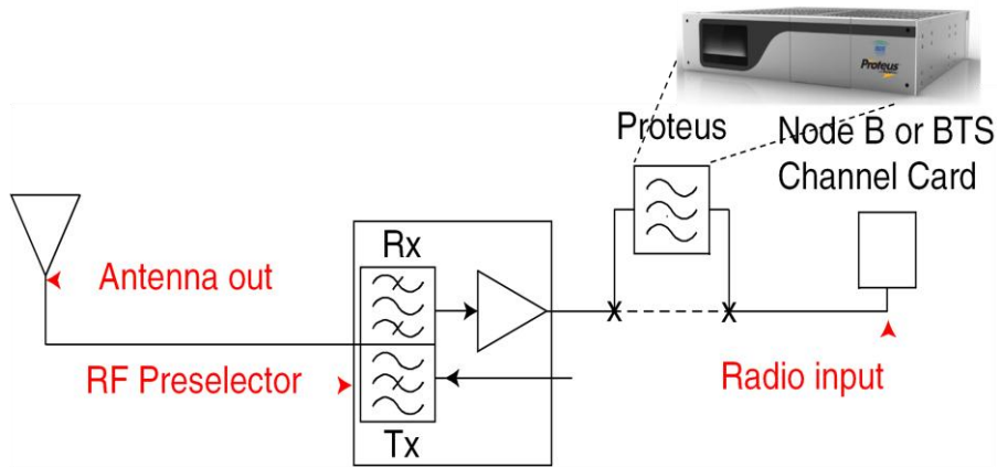
Diagram 1. Proteus installs on the receive, uplink path
